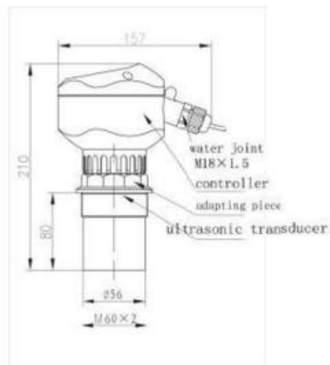
Figure 4-6 Thread of sensor (M60x2)
