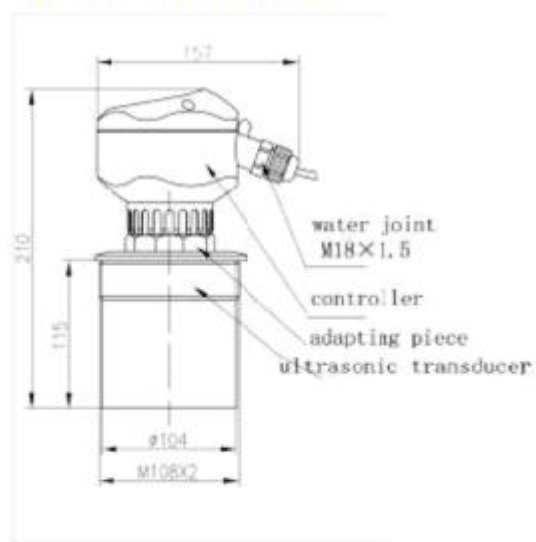
Figure 4-8 Thread of Sensor (M108x2)
