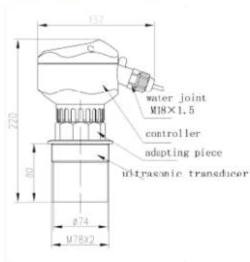
Figure 4-7 Thread of sensor (M78x2)
